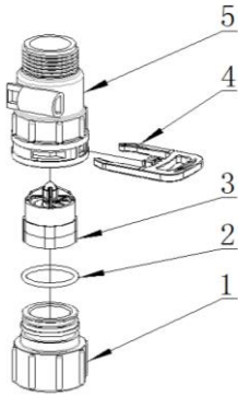
5447118 Flow Meter
